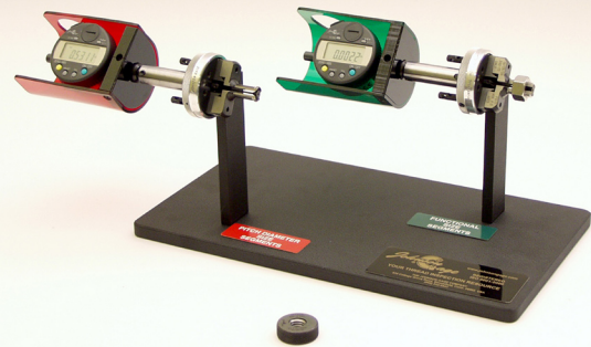
Series GJ/GJ Internal Adjustable
